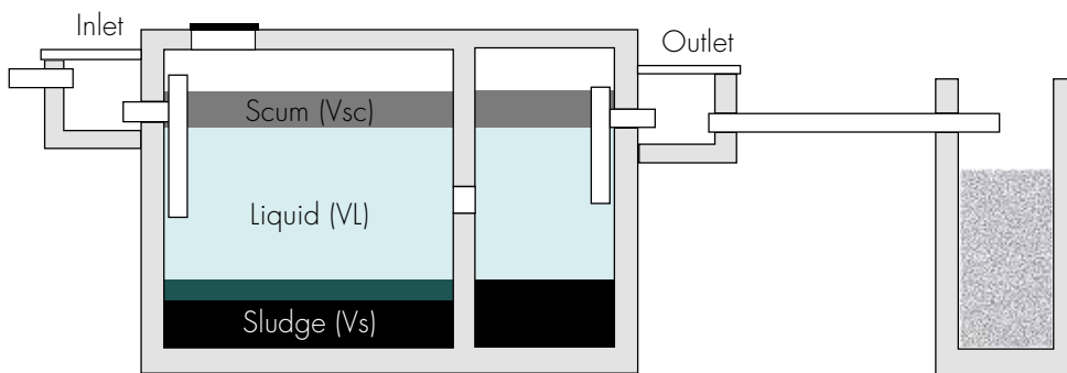
Figure 3: Volume of Septic Tank
